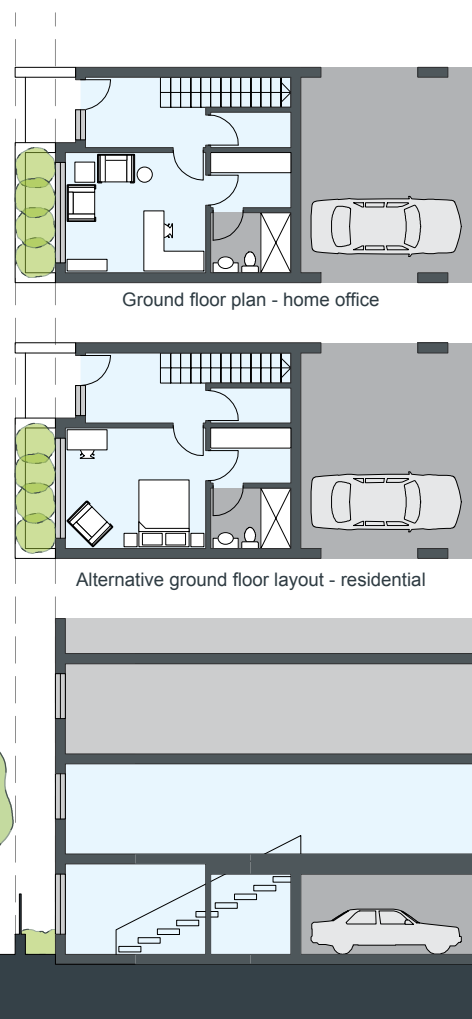
Figure 4L.3 Plan and section of a double storey apartment which is directly accessible from the street
