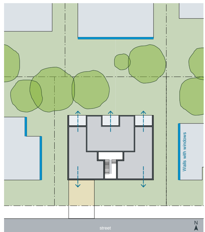
Figure 2H.2 On infill sites follow the existing open space patterns, limit side setbacks and locate habitable rooms to face the street and rear boundary to optimise amenity and privacy for all
