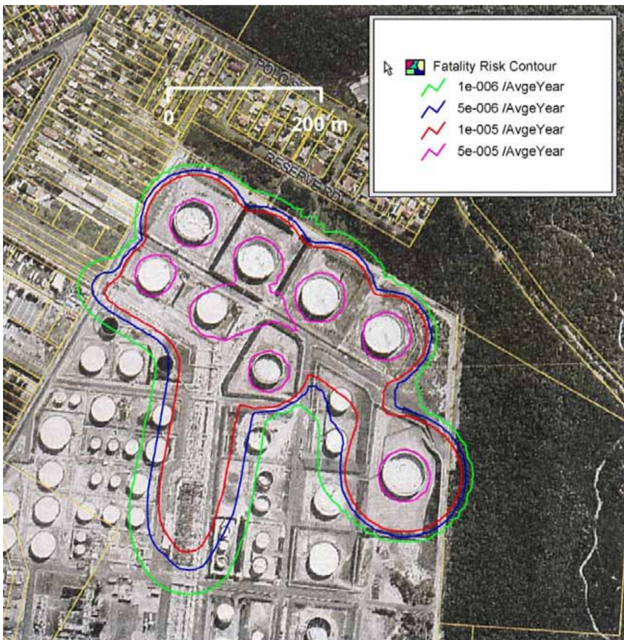
Figure 12: Individual Fatality Risk Contours
