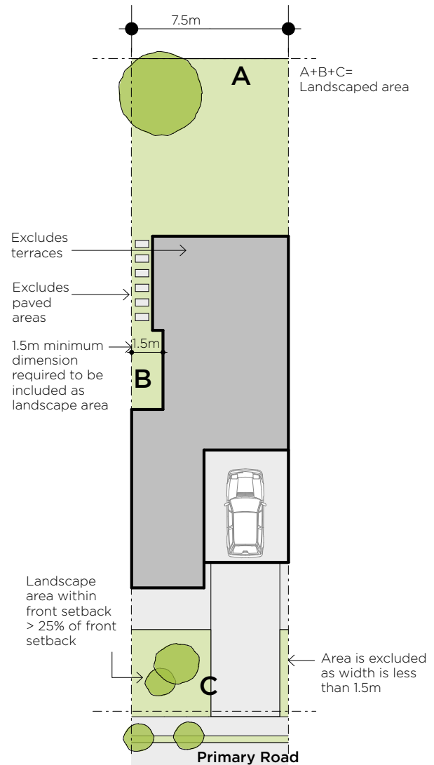
Figure 3-37 Landscaped areas distributed around the site. The minimum dimension ensures the space is sustainable for substantial planting (A+B+C = total landscape required).
