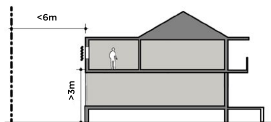
FFL above natural ground level >3m and distance to boundary is <6m Privacy screen required
