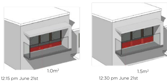
Figure 3-63 For solar access to be included, at least 1m 2 of sunlight must remain in a window for a 15 minute period
