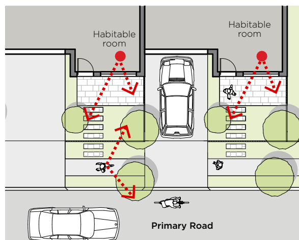
Figure 3-48 New buildings should contribute to and improve the existing streetscape. Windows and porches should be included in the street elevation to increase passive surveillance.
