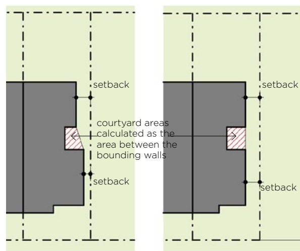
Figure 3-64 Courtyard used to increase daylight access are calculated by the areas between bounding walls
