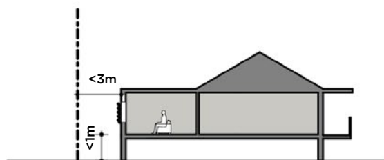
FFL above natural ground level >1m and distance to boundary is <3m Privacy screen required
