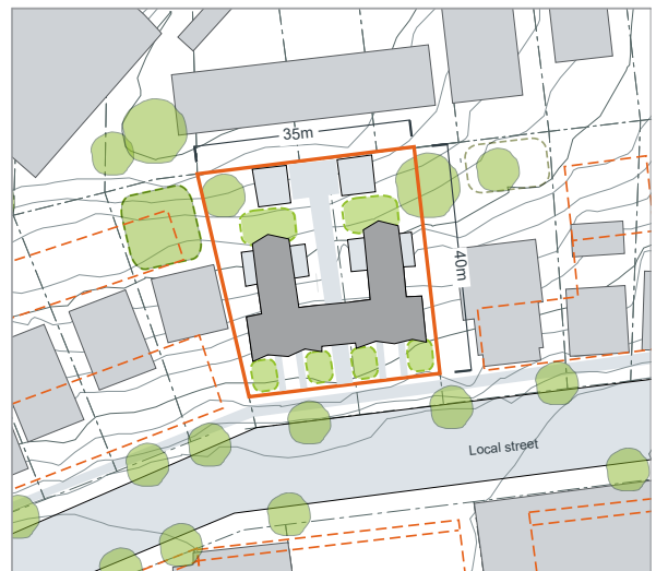
Figure 3-45 SITE SCALE: The site scale is a detailed analysis of the developments immediate context and should include the site itself, the street it addresses and surrounding properties.
