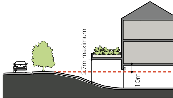
Figure 3-51 Reduce visual impact of basement entries by reducing the scale of the garage opening
