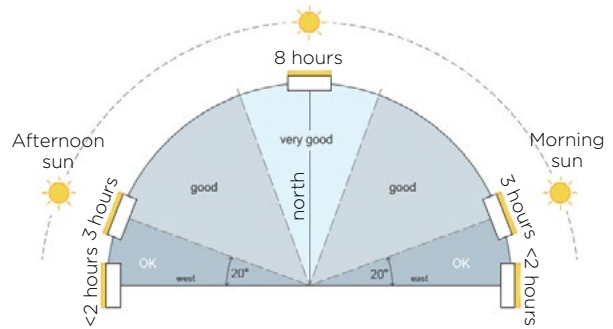
Figure 3-61 The hours of sunlight that can be expected in mid-winter are directly related to the orientation of the façade. This diagram shows the optimal orientation for habitable rooms and balconies
