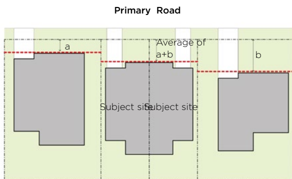
Figure 3-32 Primary road setback
