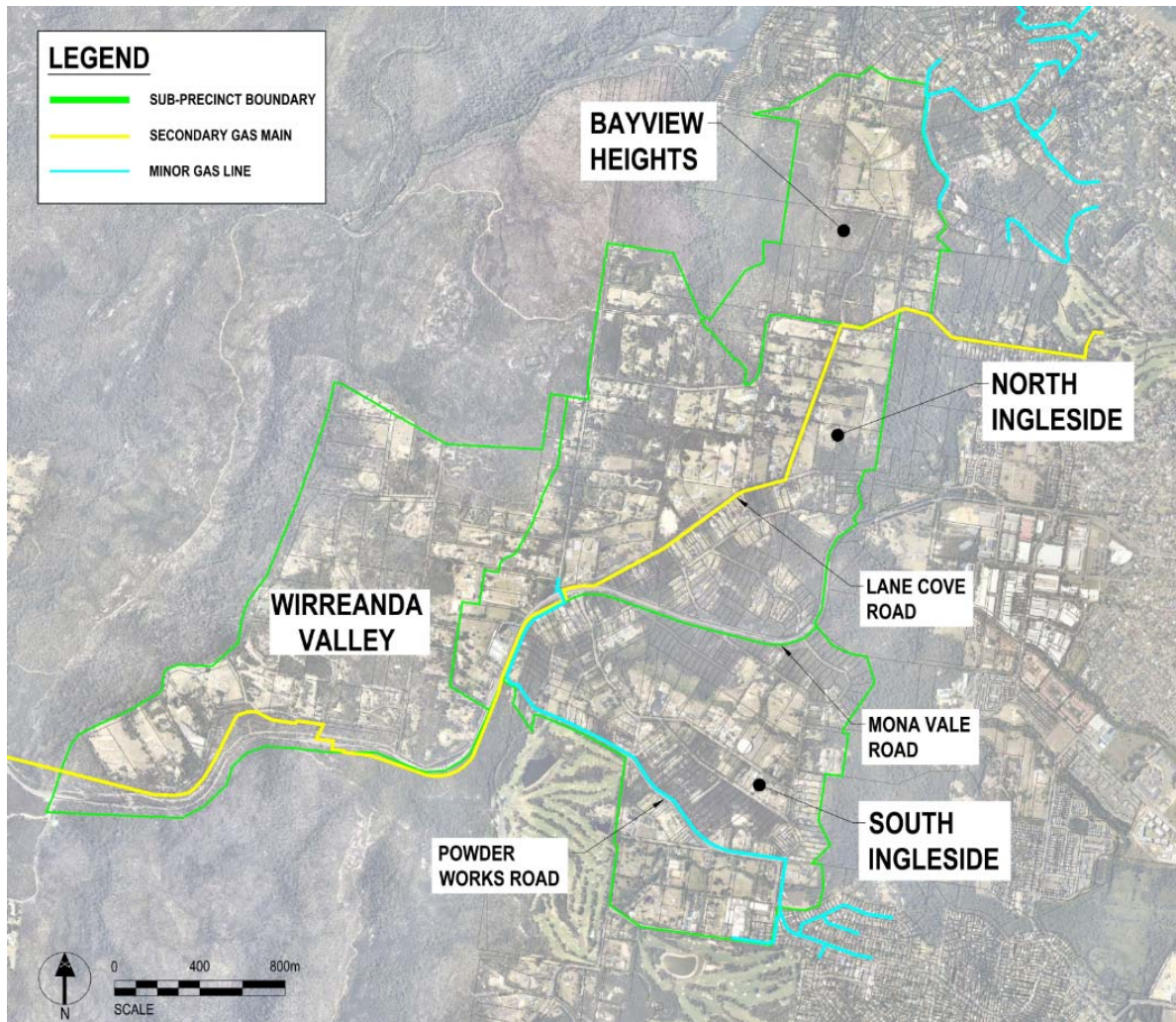
Figure 3-5 Existing Gas Infrastructure
